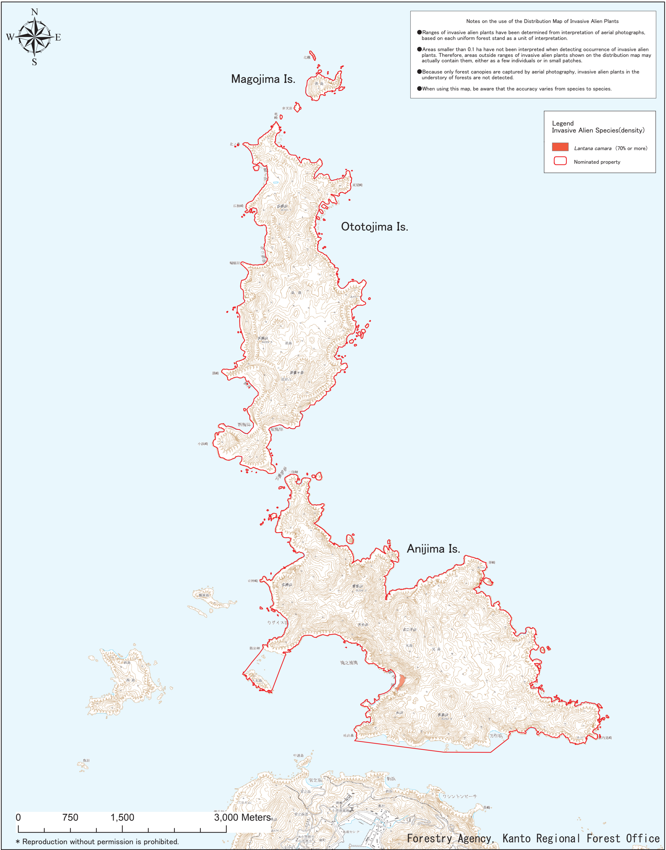
Fig. 3-3 Distribution Map of Invasive Alien Plants on the Ogasawara Islands Anijima Island Ototojima Island Magojima Island
